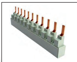
Closed busbar system L1 – L2 – L1 – L2
