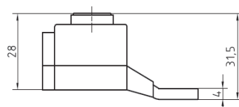
Feed-in terminal 95mm 2 , Pin for load-switch
